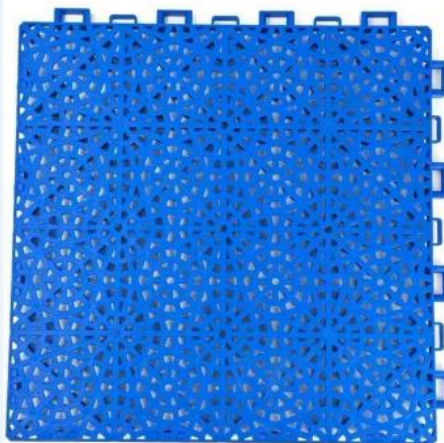
Pattern 1 Spec: 300x300x13(mm)
