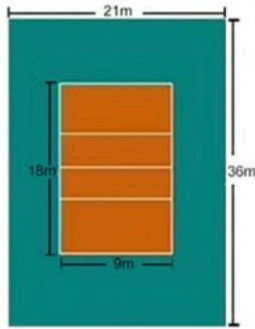
Volleyball court
